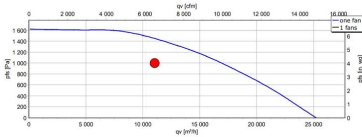
Air performance
